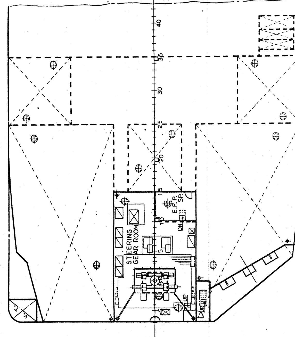
STEERING GEAR FLAT
