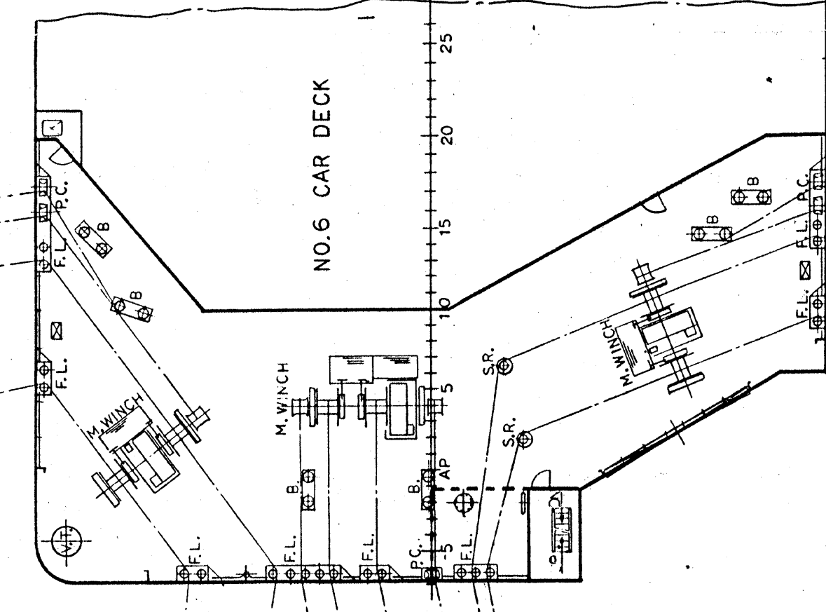
AFT MOORING DECK (NO. 5 CAR DECK)
