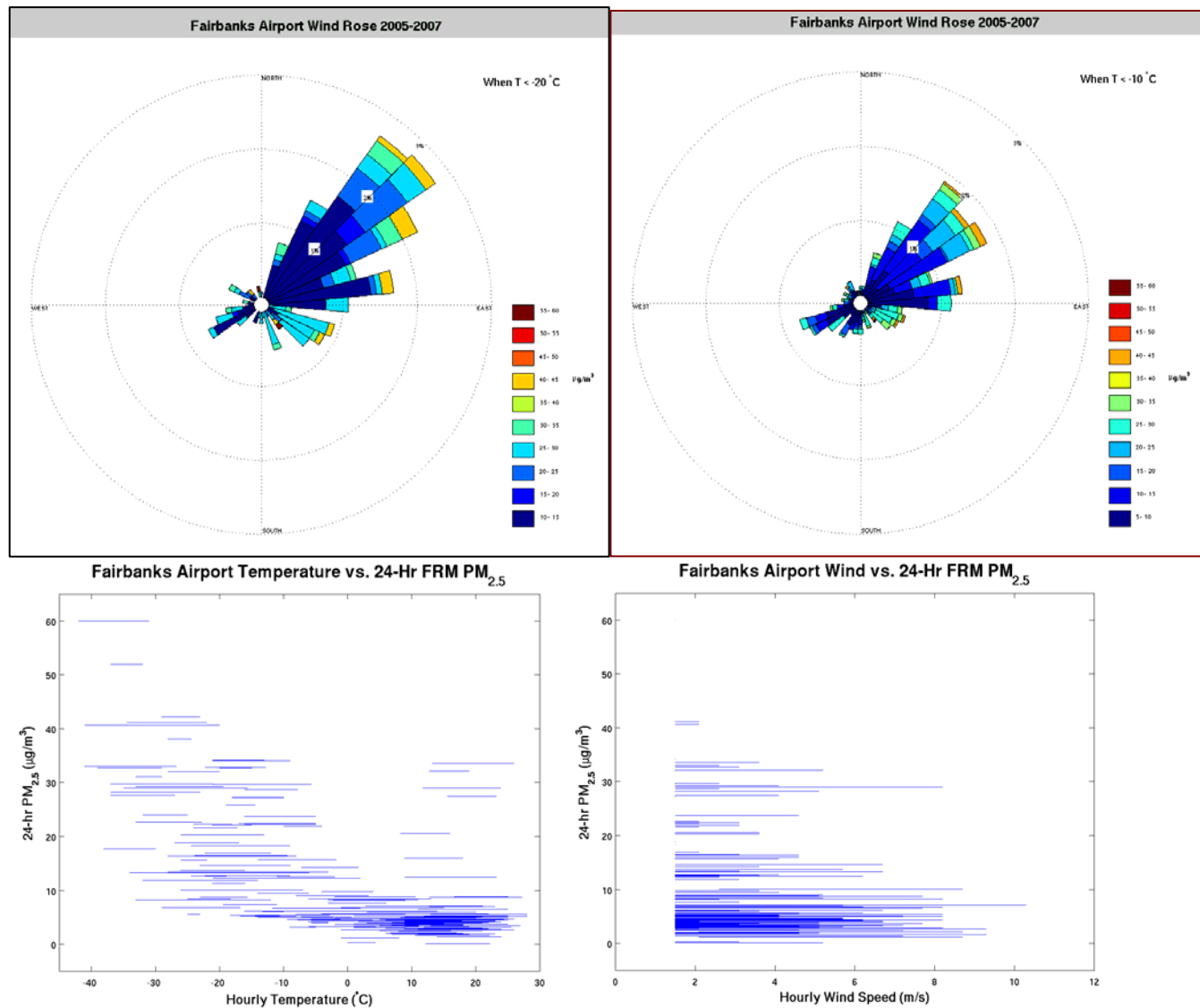
Figure 11: Temperature and pollution rose plots form Fairbanks, 2005-2007.
